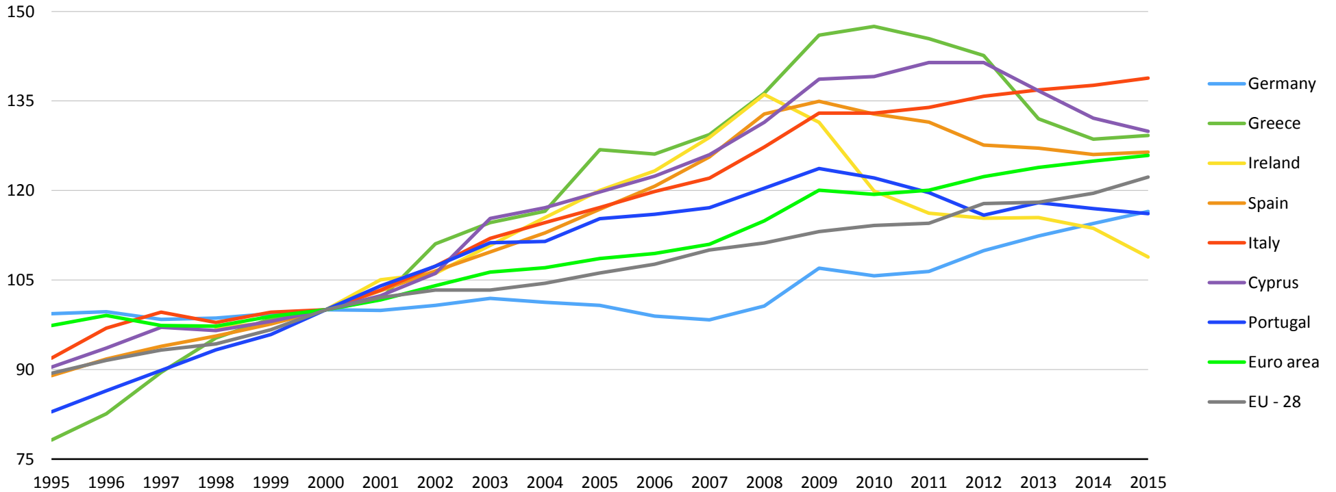
Figure: Unit labour cost (2000=100, total economy, 1995-2015)
