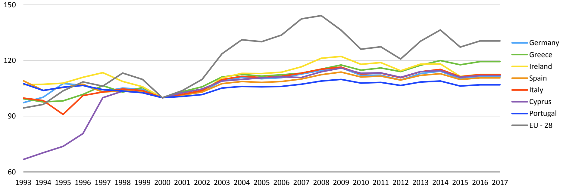
Figure: Nominal effective exchange rate (2000=100, performance relative to the other 37 industrial countries, 1993-2017)
